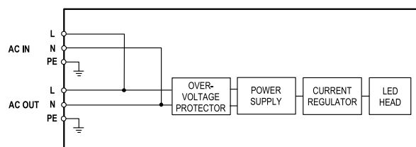
LI-10-115-F block diagram
